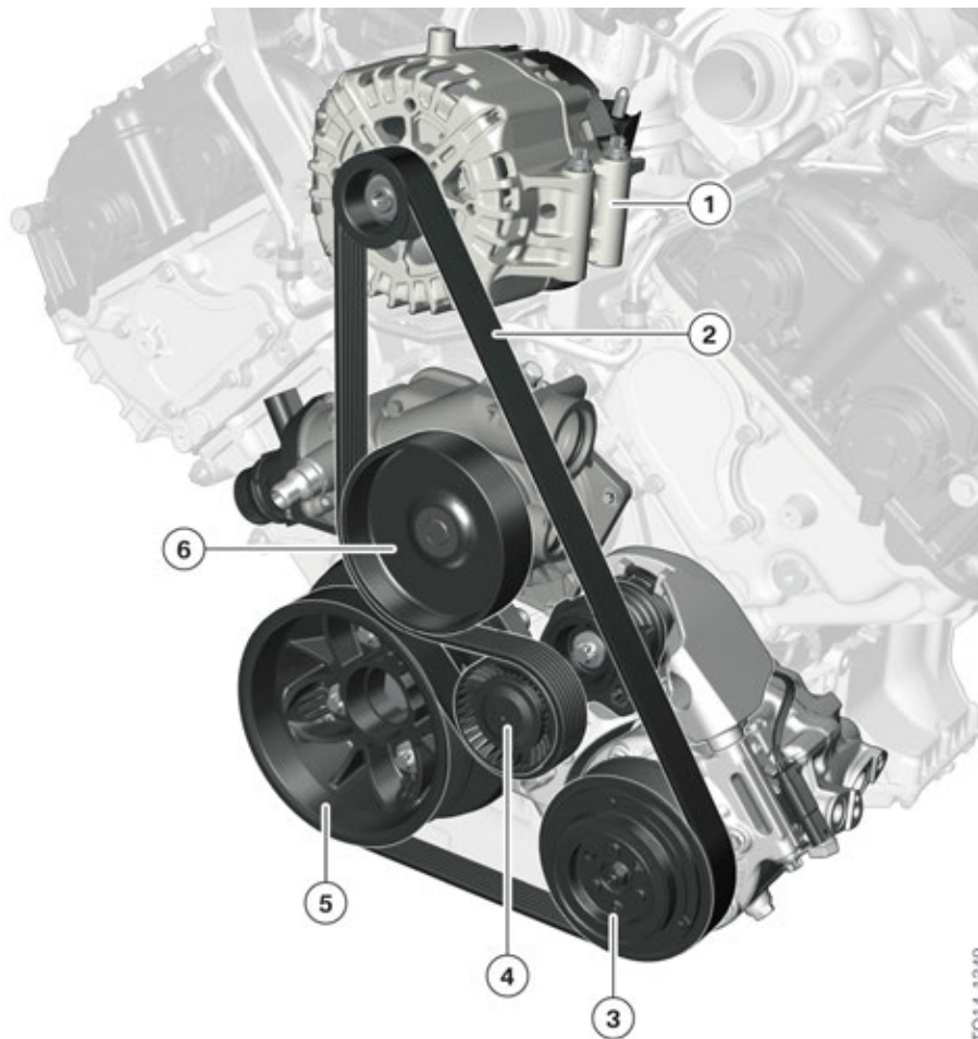
N63TU2 engine, belt drive
